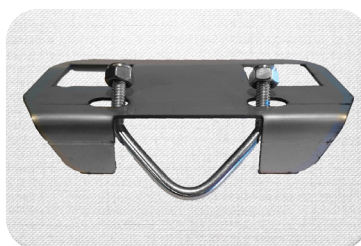
Angle top mounting hardware
